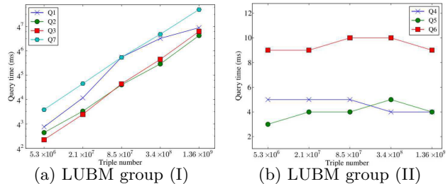
Figure 8: Data scalability
