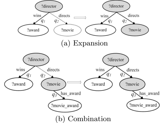
Figure 7: Expansion and combination examples
