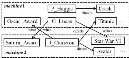
Figure 6: Distribution of the RDF graph in Figure 1
