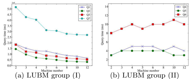
Figure 9: Machine scalability
